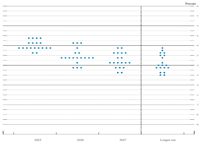
Dot Plot (March 2025)
